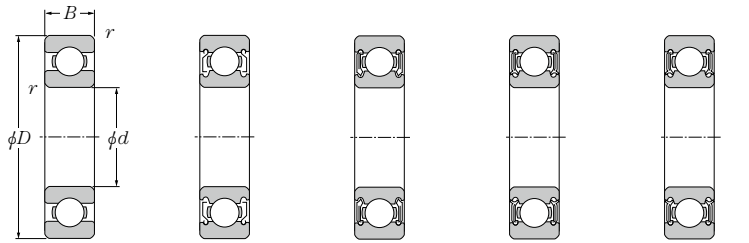
Open type Shielded type (ZZ) Non-contact sealed type (LLB) Low torque sealed type (LLH) Contact sealed type (LLU)
