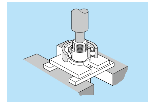
Fig. 15.29 Press disassembly
