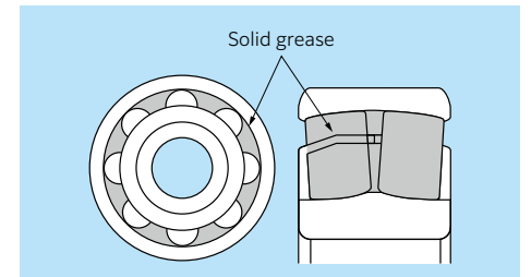
Fig. 11.4 Spherical roller bearing with full-pack solid grease (Available for spherical roller bearings)
