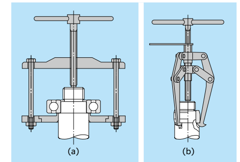
Fig. 15.28 Puller disassembly
