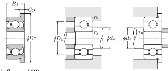
With flanged OR and double shield (FL...ZZ)
