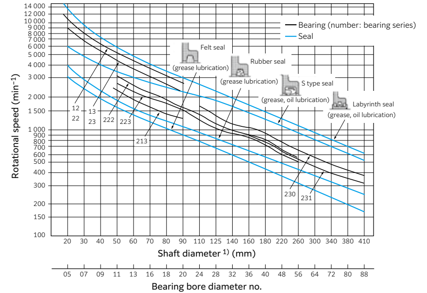
1) The allowable speed of the seal of cylindrical bore bearings is obtained by the shaft diameter of the seal contact part. The allowable speed of seals is indicated by the rotational speed of shafts.
