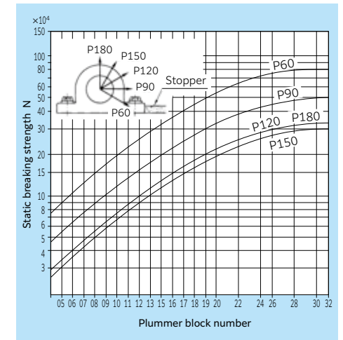
Fig. 10 Static breaking strength of SN6 series
