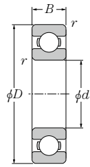
Open type
