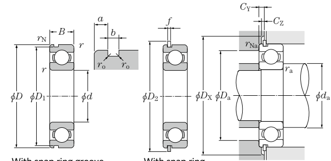
With snap ring groove
