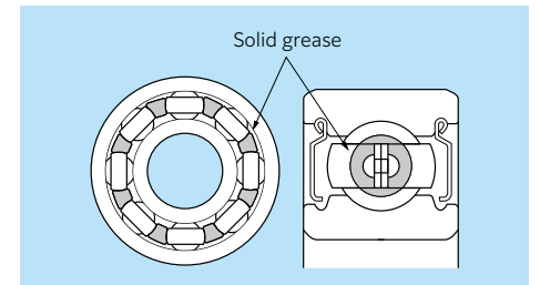
Fig. 11.3 Deep groove ball bearing with spot-pack solid grease (Z shield) (Available for deep groove ball bearings)
